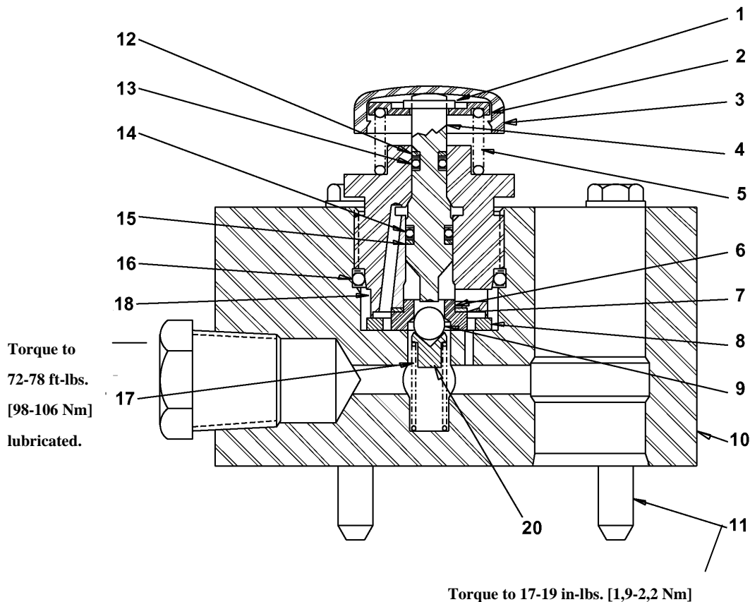
Figure 9 - Release Valve
