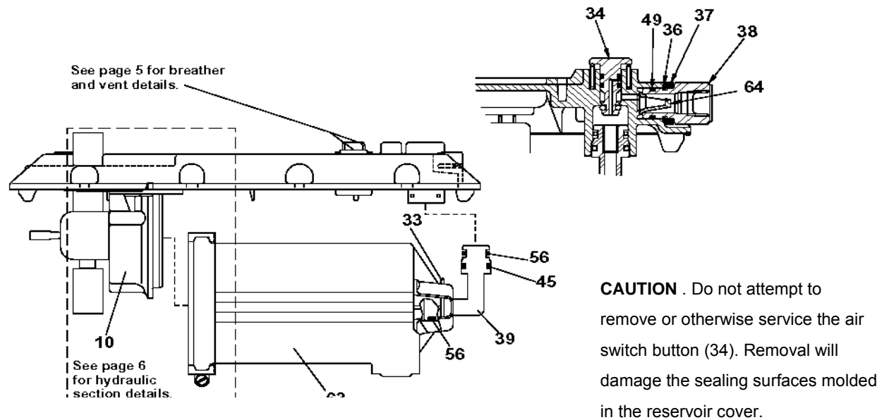
Figure 3 - Cover Assembly Side View
