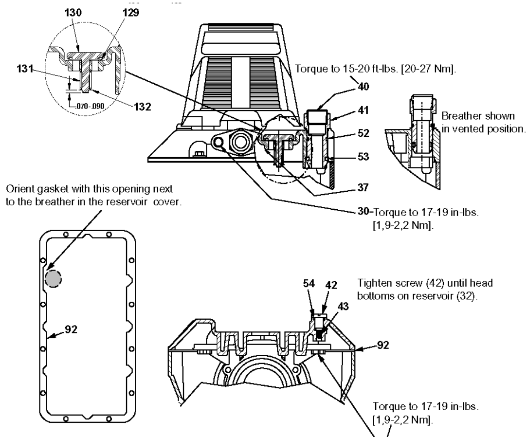
Figure 5 - Reservoir End View
